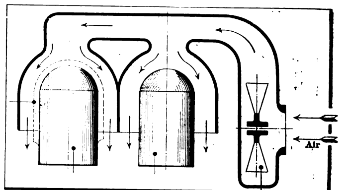
Fig. 60—Air-blast, through the use of a fan; may be adopted in conjunction with exhaust energy in the cooling process
